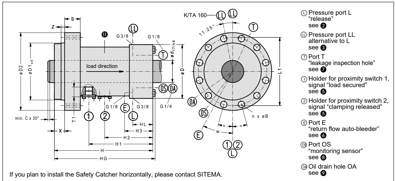
Fig. 2: Dimensions of Safety Catcher K/TA (download CAD files from www.sitema.com)
